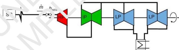
Figure 7 Turbine, divided into sections. First section: high pressure (HP); second section: intermediate pressure (IP), double flow; third section: low pressure (LP), tandem double flow.
