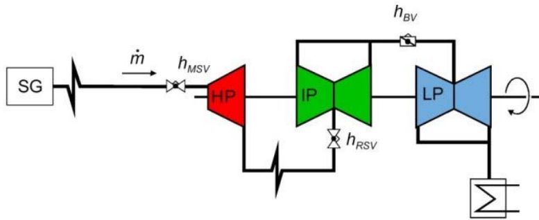
Figure 8. Reheating after the HP section
