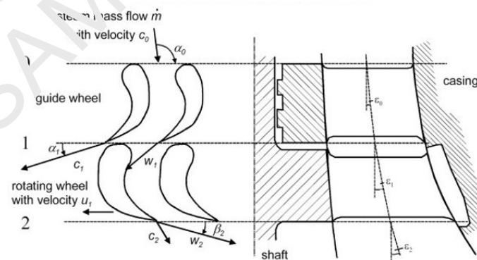
Figure 6. Guide wheel and rotating wheel. c_i : absolute velocities; w_i : velocities relative to the rotating wheel
