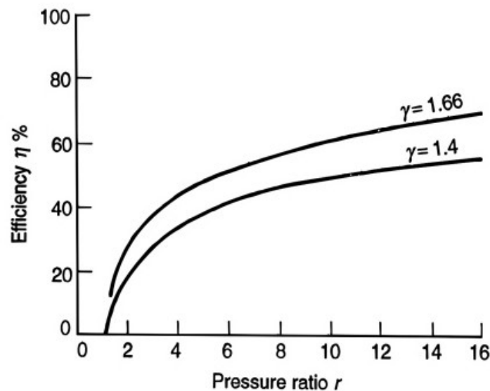
Figure 4. Efficiency for simple cycle
