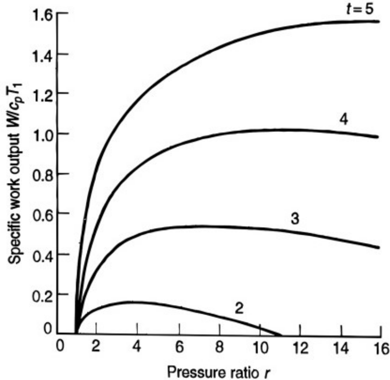
Figure 5. Specific work output for simple cycle
