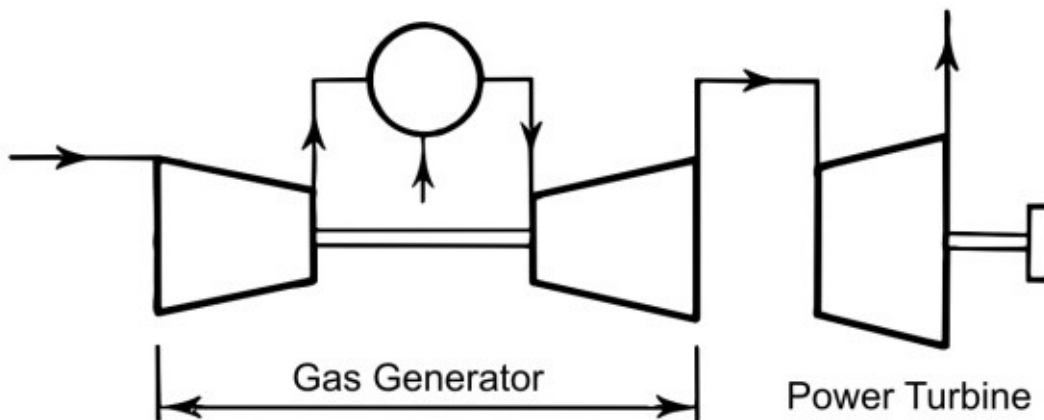
Figure 2. Gas turbine with separate power turbine
