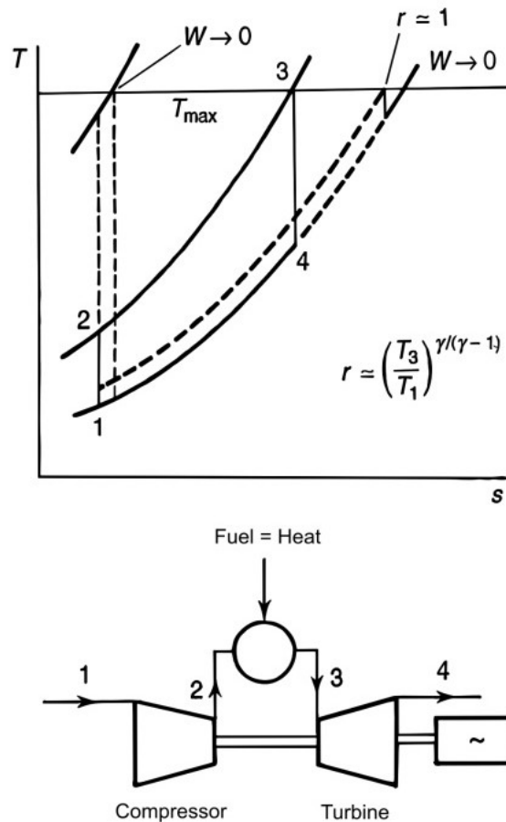
Figure 3. Simple cycle
