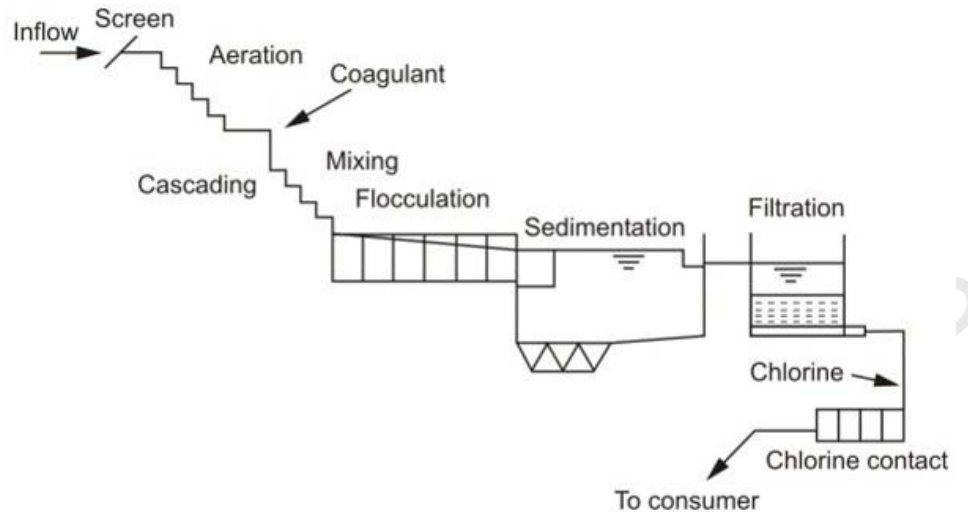
Figure 1. Diagrammatic layout of typical water purification plant
